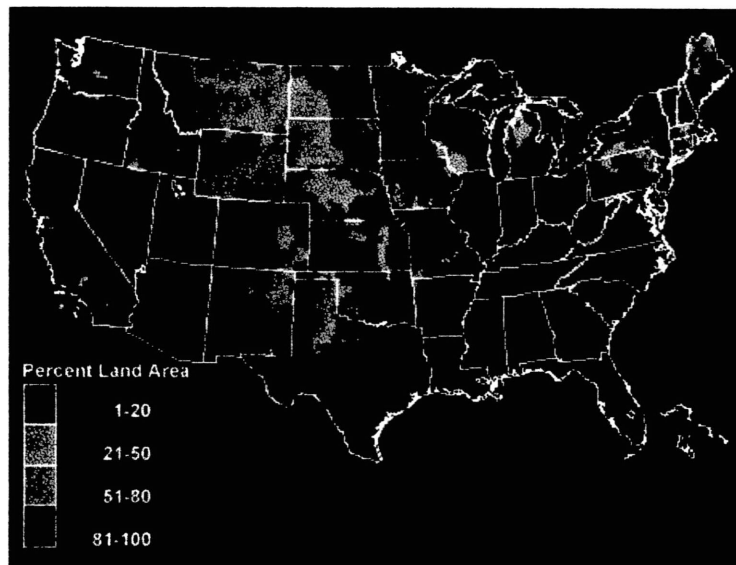
Figure 2. Percent U.S. Land Area with Wind Resource Class 3 or Above (Annual)
