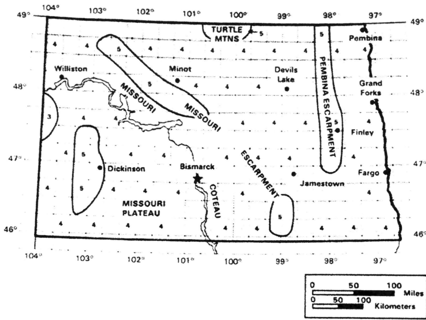
3-12 North Dakota annual average wind power
