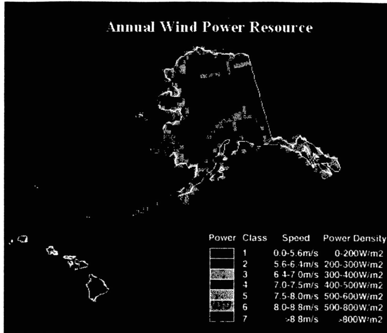
Figure 1a. Annual Wind Power Resource Alaska and Hawaii
